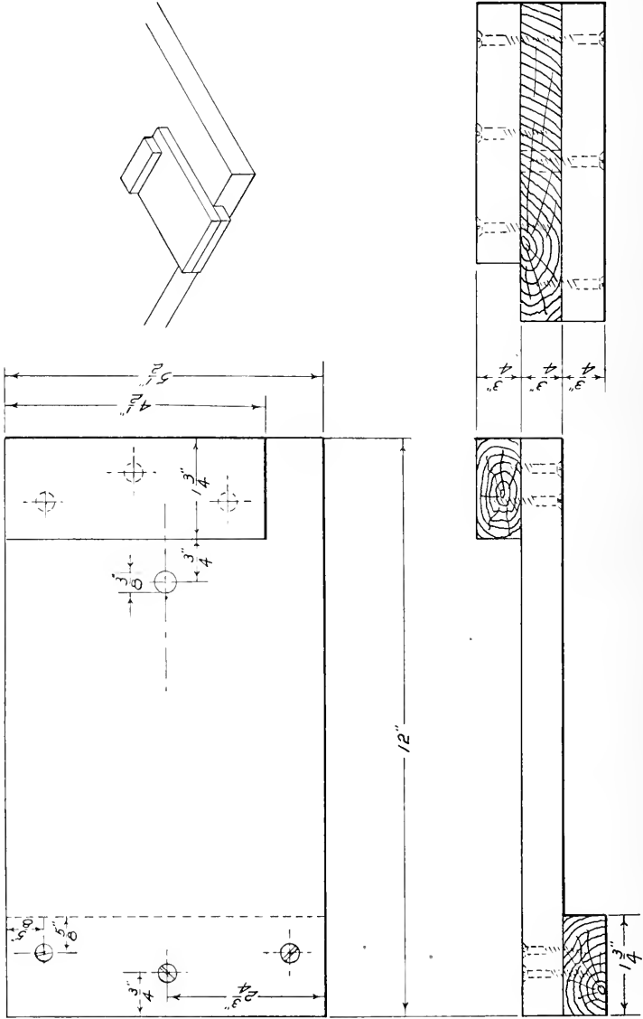
Bench Hook
